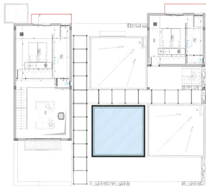
PLAN - 1 ST FLOOR
